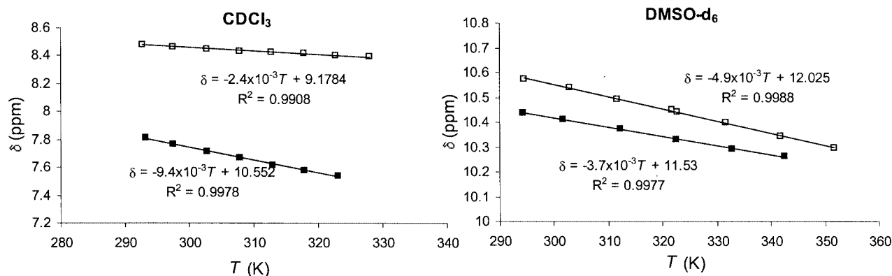
Figure 1. Temperature dependence of 1 H NMR chemical shifts for the amido protons of 3- Z (□) and 3- E (■) in CDCl 3 and [D 6 ]DMSO
