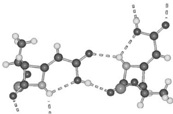
Figure 3. A view of the molecular compound 23 ; for the sake of clarity, the alkyl substituents of the silicon atom (wider atom) are omitted; the hydrogen bonds are shown as dotted lines
