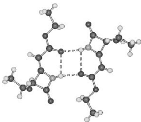
Figure 2. A view of the molecular compound 22 ; the hydrogen bonds are shown as dotted lines
