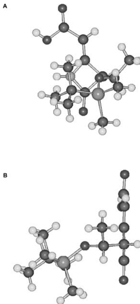
Figure 4. Two views of the molecular compound 23 showing the TBS protecting group; in A, the plane of the \beta -lactam ring is perpendicular to the view direction; in B, it is parallel
